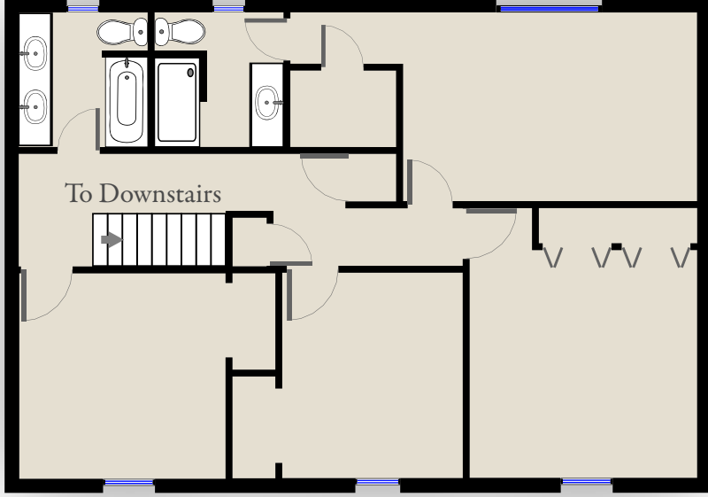
Second Floor
